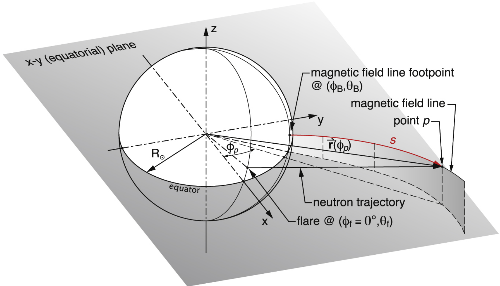
Figure 7. from Neutron-decay Protons from Solar Flares as Seed Particles for CME-shock Acceleration in the Inner Heliosphere null 2017 APJ 846 53 doi:10.3847/1538-4357/aa7fb3 https://dx.doi.org/10.3847/1538-4357/aa7fb3 © 2017. The American Astronomical Society. All rights reserved.
