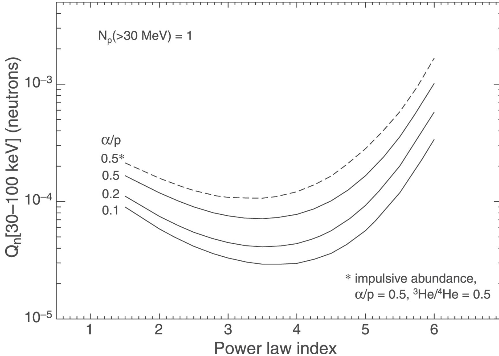
Figure 5. from Neutron-decay Protons from Solar Flares as Seed Particles for CME-shock Acceleration in the Inner Heliosphere null 2017 APJ 846 53 doi:10.3847/1538-4357/aa7fb3 https://dx.doi.org/10.3847/1538-4357/aa7fb3 © 2017. The American Astronomical Society. All rights reserved.
