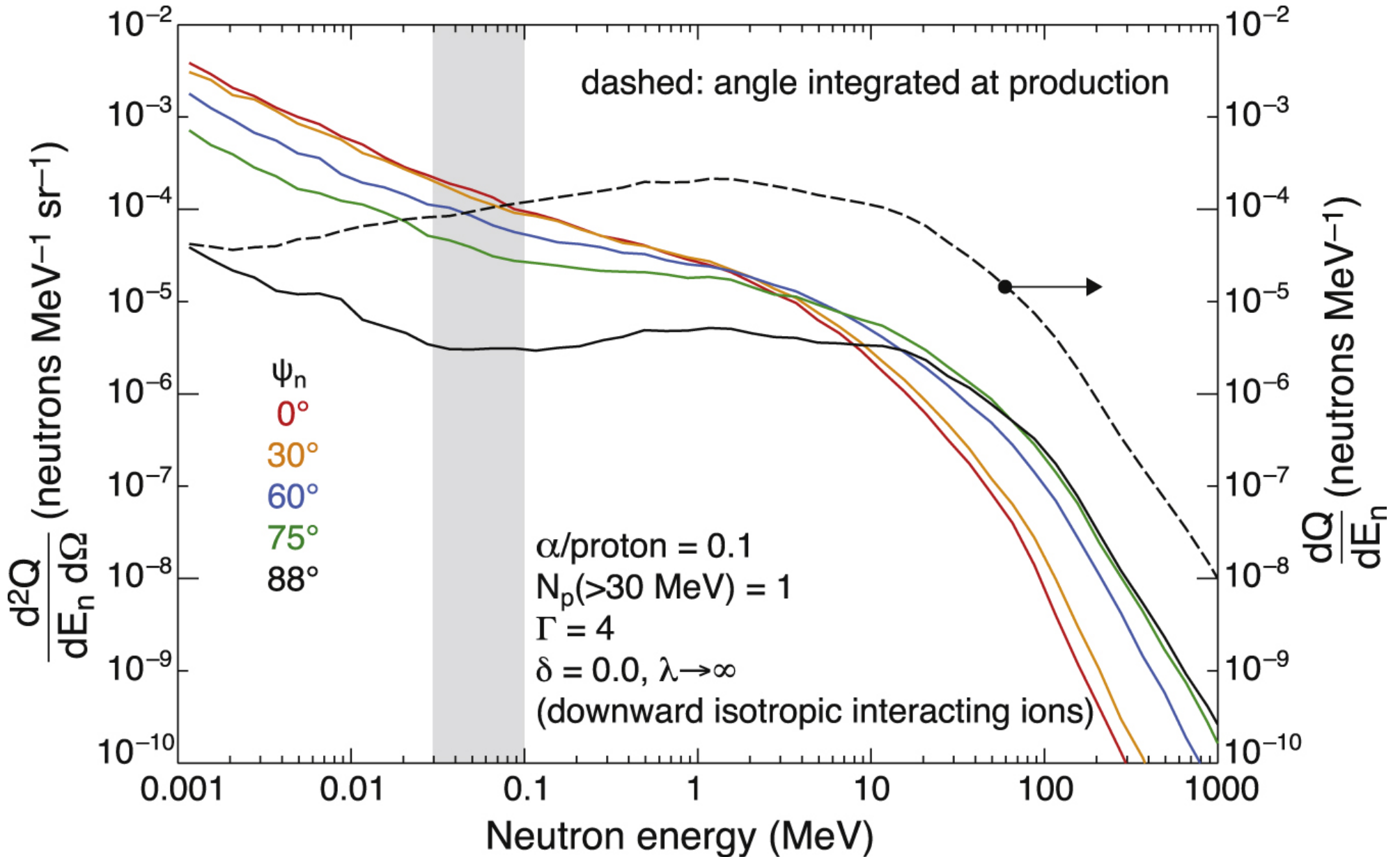
Figure 4. from Neutron-decay Protons from Solar Flares as Seed Particles for CME-shock Acceleration in the Inner Heliosphere null 2017 APJ 846 53 doi:10.3847/1538-4357/aa7fb3 https://dx.doi.org/10.3847/1538-4357/aa7fb3 © 2017. The American Astronomical Society. All rights reserved.
