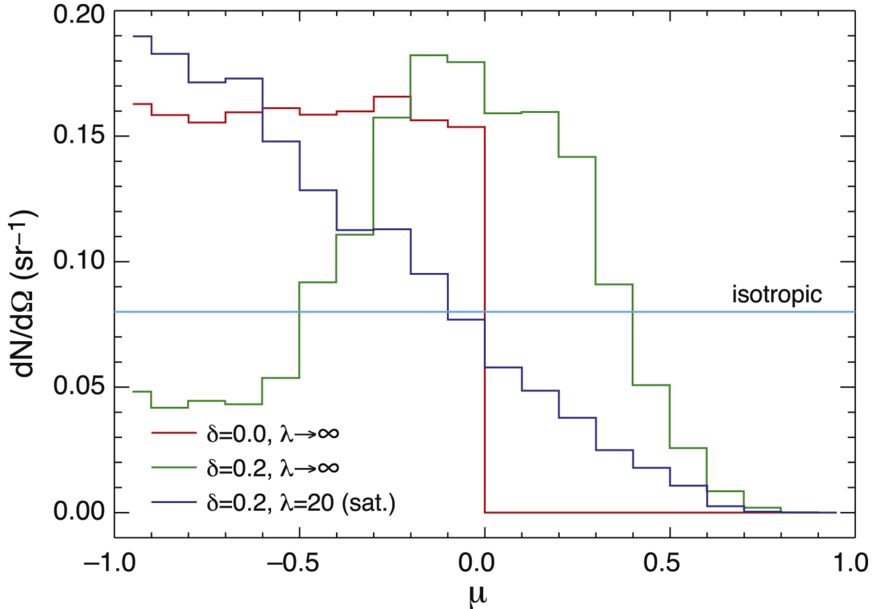
Figure 2. from Neutron-decay Protons from Solar Flares as Seed Particles for CME-shock Acceleration in the Inner Heliosphere null 2017 APJ 846 53 doi:10.3847/1538-4357/aa7fb3 https://dx.doi.org/10.3847/1538-4357/aa7fb3 © 2017. The American Astronomical Society. All rights reserved.
