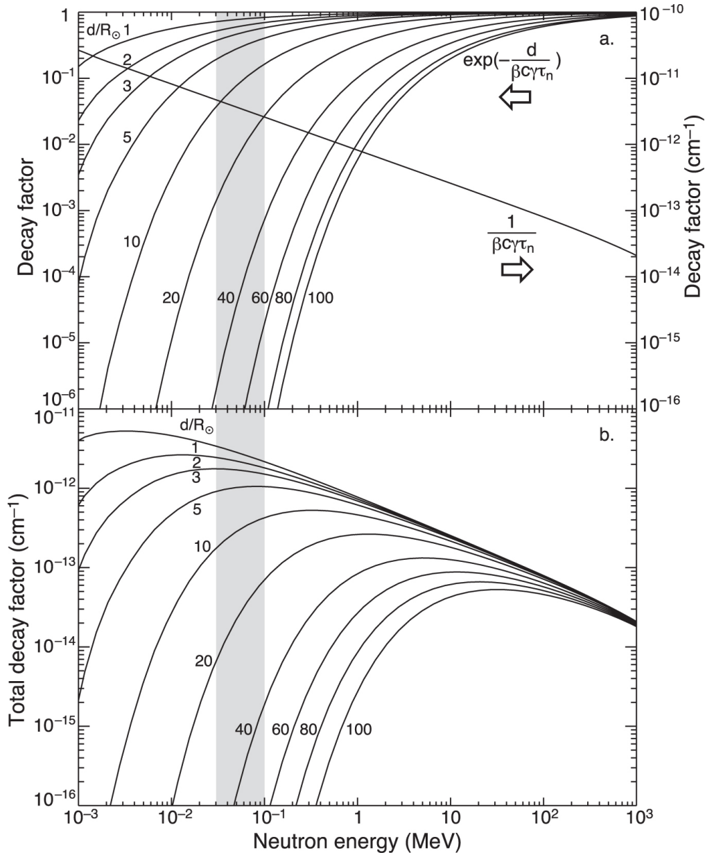
Figure 14. from Neutron-decay Protons from Solar Flares as Seed Particles for CME-shock Acceleration in the Inner Heliosphere null 2017 APJ 846 53 doi:10.3847/1538-4357/aa7fb3 https://dx.doi.org/10.3847/1538-4357/aa7fb3 © 2017. The American Astronomical Society. All rights reserved.
