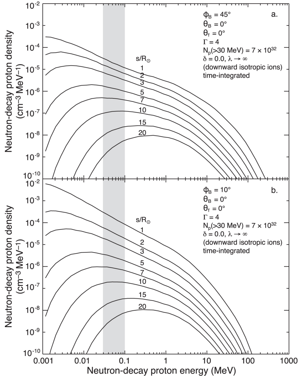
Figure 13. from Neutron-decay Protons from Solar Flares as Seed Particles for CME-shock Acceleration in the Inner Heliosphere null 2017 APJ 846 53 doi:10.3847/1538-4357/aa7fb3 https://dx.doi.org/10.3847/1538-4357/aa7fb3
