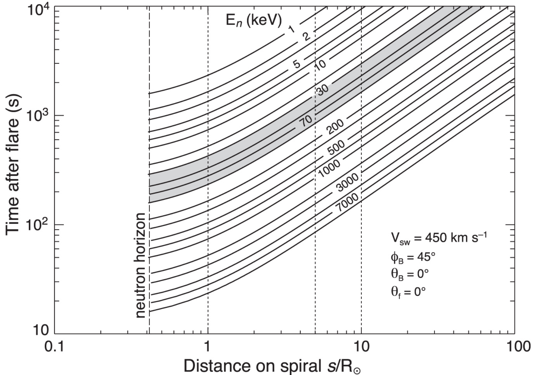
Figure 12. from Neutron-decay Protons from Solar Flares as Seed Particles for CME-shock Acceleration in the Inner Heliosphere null 2017 APJ 846 53 doi:10.3847/1538-4357/aa7fb3 https://dx.doi.org/10.3847/1538-4357/aa7fb3 © 2017. The American Astronomical Society. All rights reserved.
