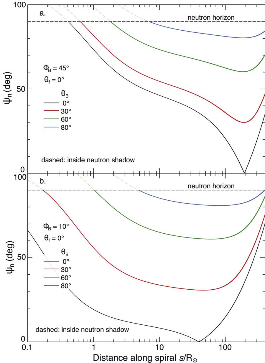
Figure 11. from Neutron-decay Protons from Solar Flares as Seed Particles for CME-shock Acceleration in the Inner Heliosphere null 2017 APJ 846 53 doi:10.3847/1538-4357/aa7fb3 https://dx.doi.org/10.3847/1538-4357/aa7fb3 © 2017. The American Astronomical Society. All rights reserved.
