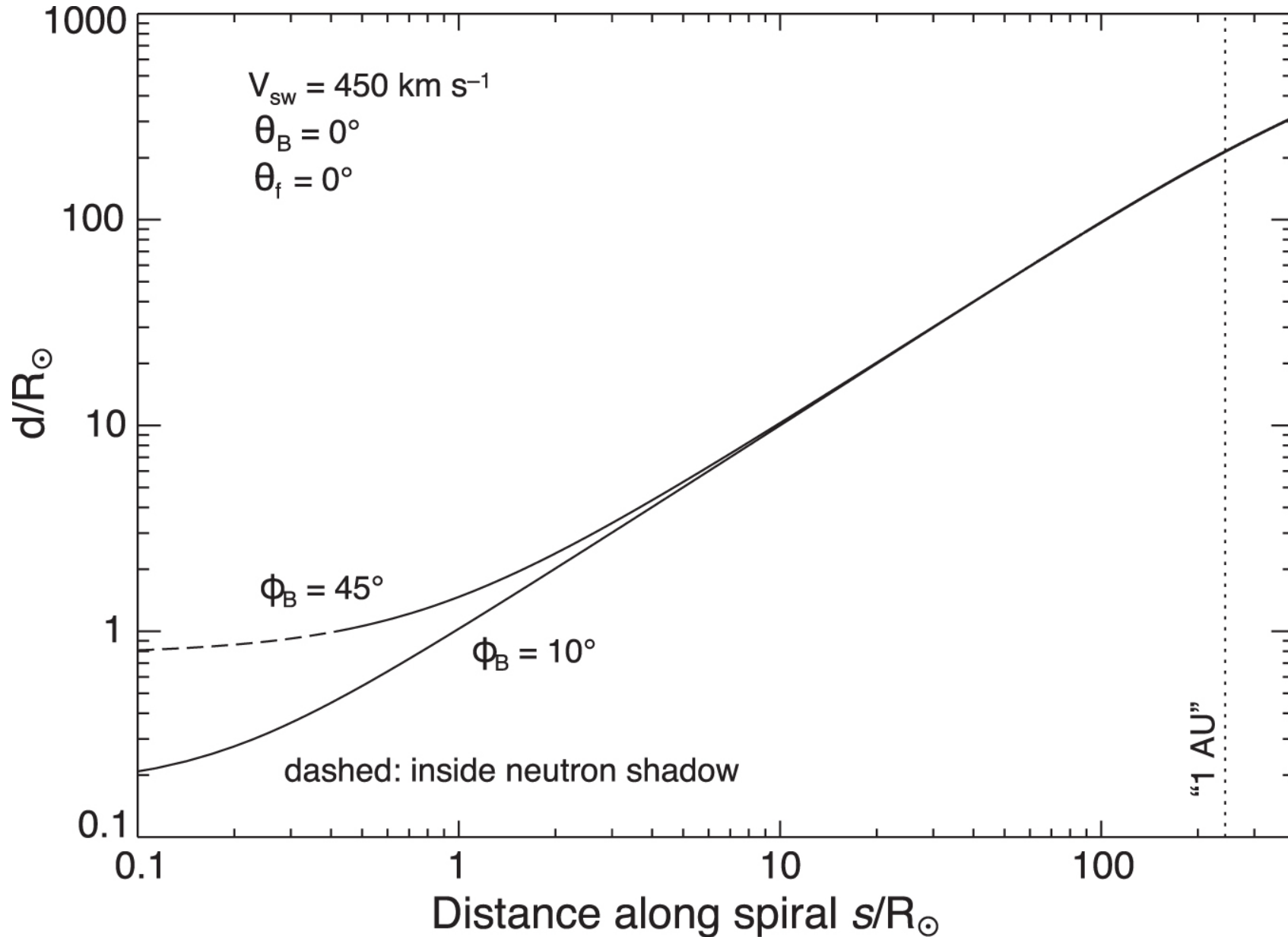
Figure 10. from Neutron-decay Protons from Solar Flares as Seed Particles for CME-shock Acceleration in the Inner Heliosphere null 2017 APJ 846 53 doi:10.3847/1538-4357/aa7fb3 https://dx.doi.org/10.3847/1538-4357/aa7fb3 © 2017. The American Astronomical Society. All rights reserved.
