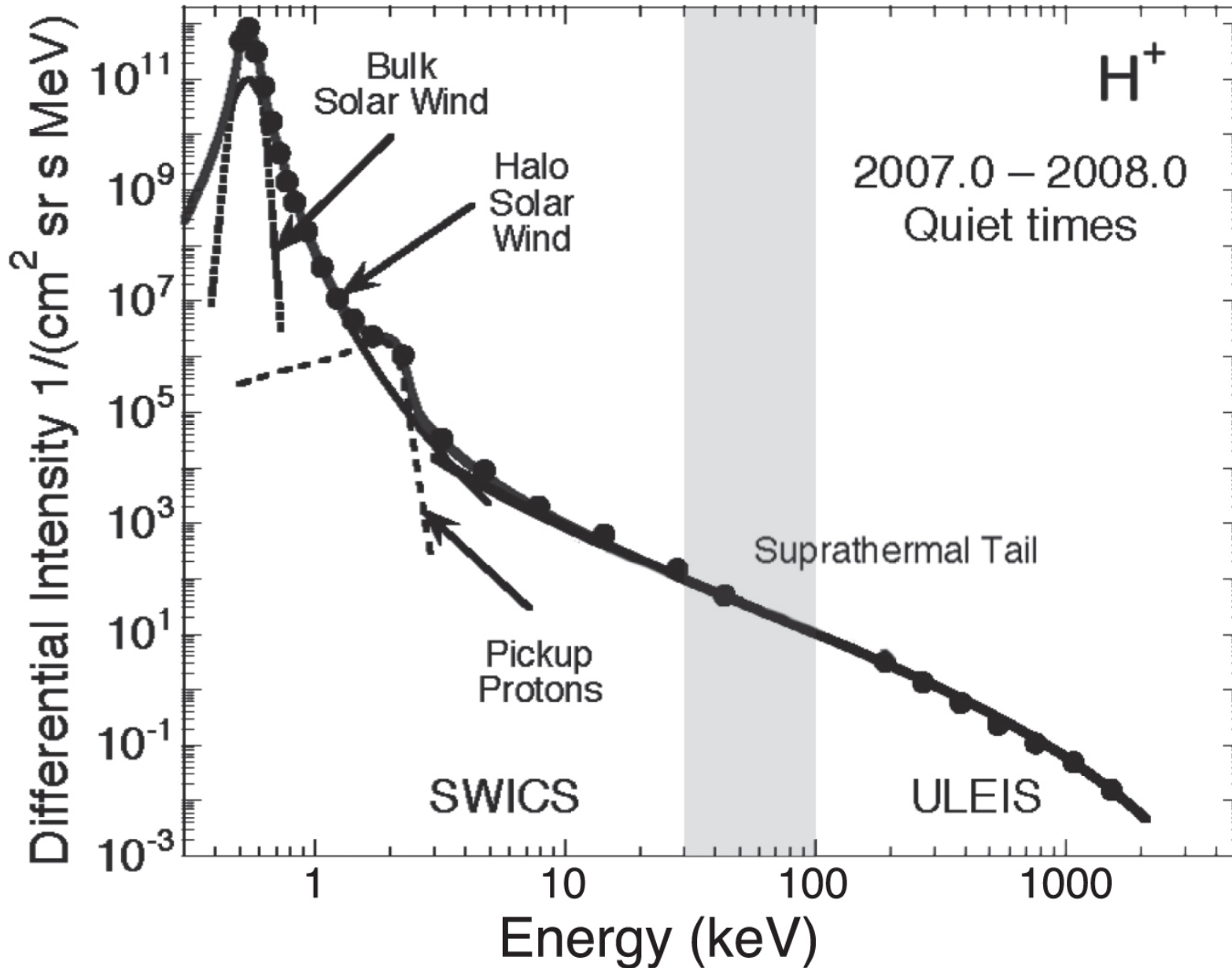
Figure 1. from Neutron-decay Protons from Solar Flares as Seed Particles for CME-shock Acceleration in the Inner Heliosphere null 2017 APJ 846 53 doi:10.3847/1538-4357/aa7fb3 https://dx.doi.org/10.3847/1538-4357/aa7fb3 © 2017. The American Astronomical Society. All rights reserved.
