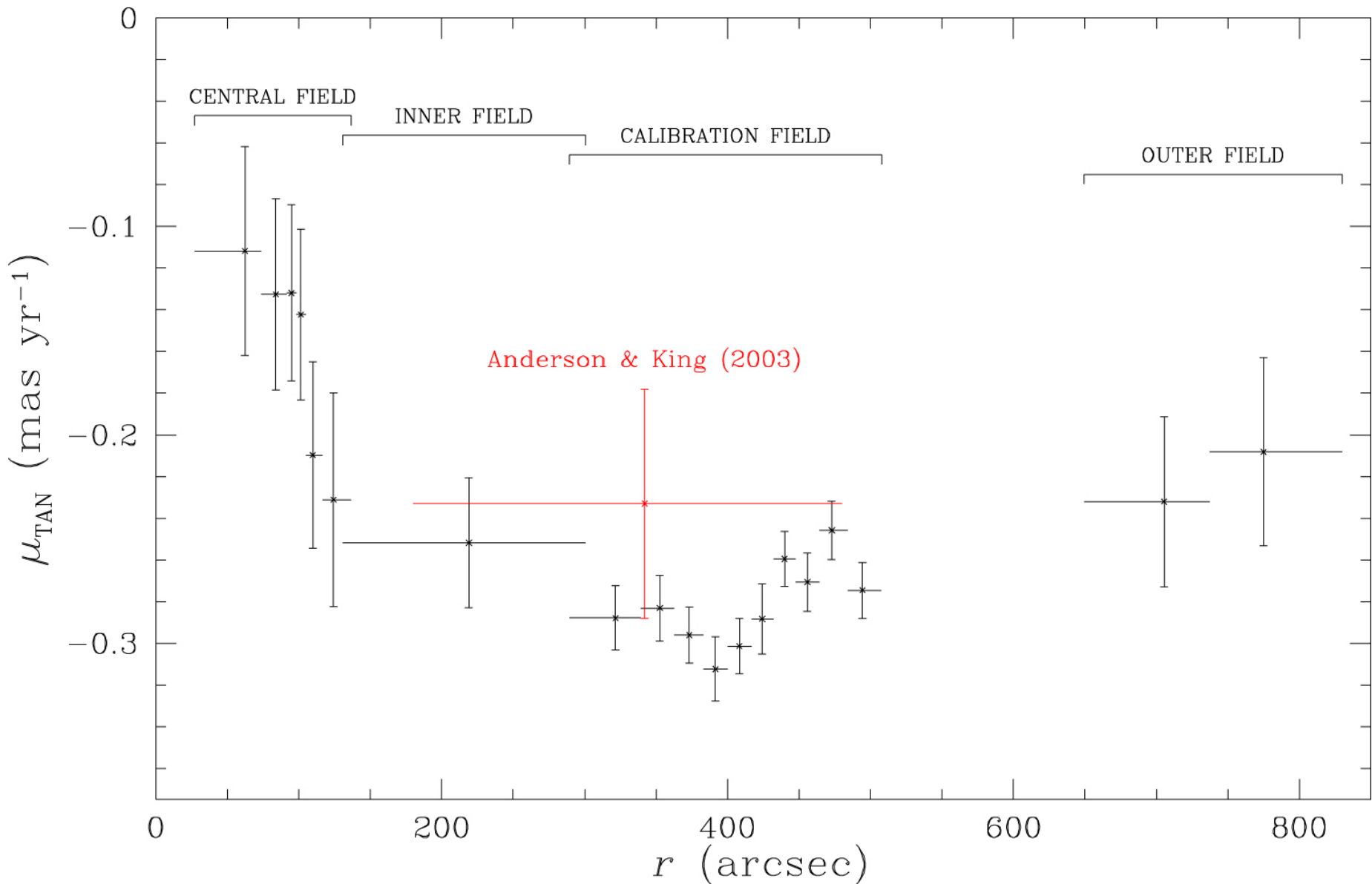
Figure 3. from Hubble Space Telescope Proper Motion (HSTPROMO) Catalogs of Galactic Globular Clusters. V. The Rapid Rotation of 47 Tuc Traced and Modeled in Three Dimensions null 2017 APJ 844 167 doi:10.3847/1538-4357/aa7c5f https://dx.doi.org/10.3847/1538-4357/aa7c5f © 2017. The American Astronomical Society. All rights reserved.
