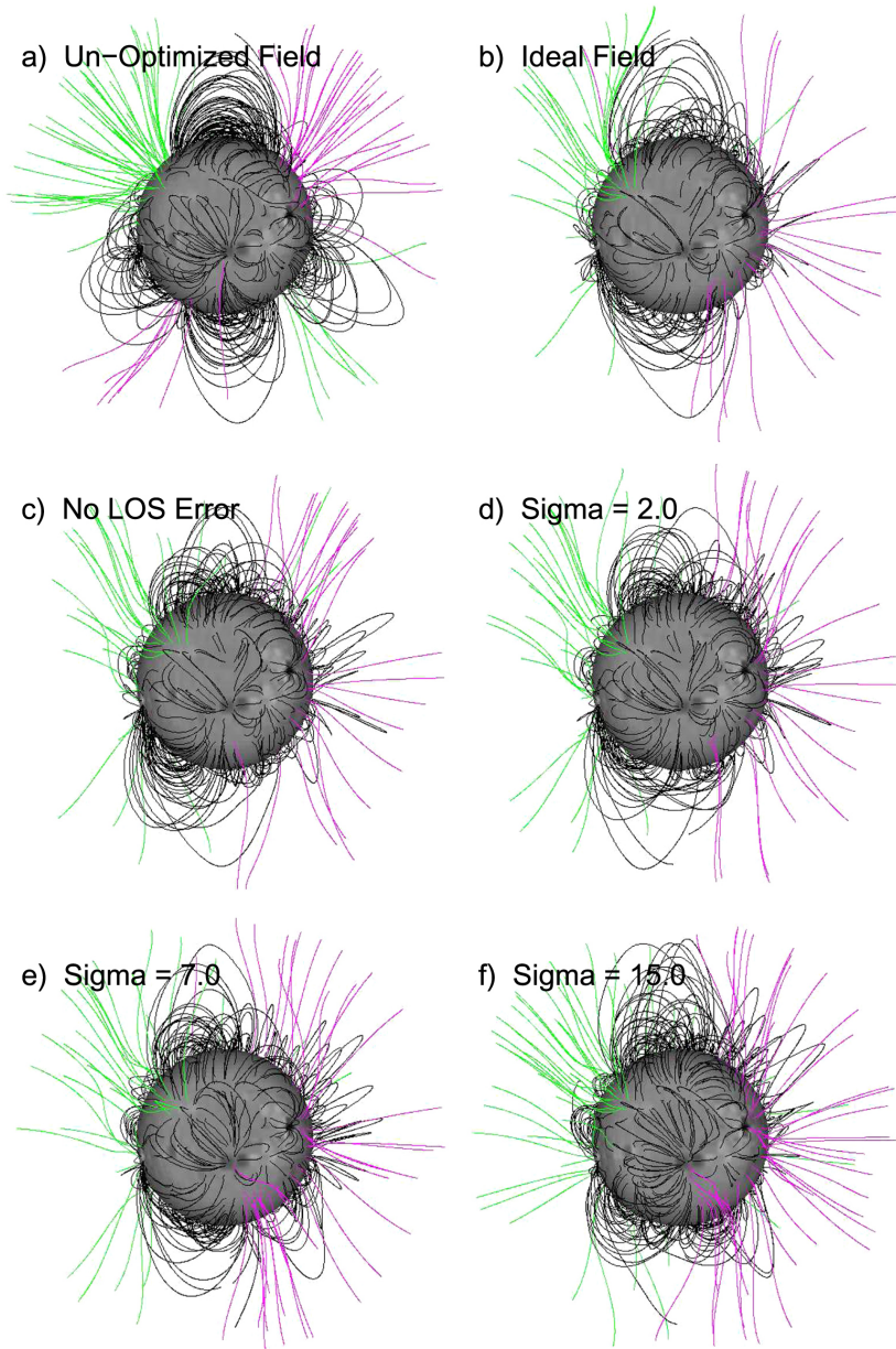
Figure 3. from Image-optimized Coronal Magnetic Field Models null 2017 APJ 844 93 doi:10.3847/1538-4357/aa7b7a https://dx.doi.org/10.3847/1538-4357/aa7b7a © 2017. The American Astronomical Society. All rights reserved.
