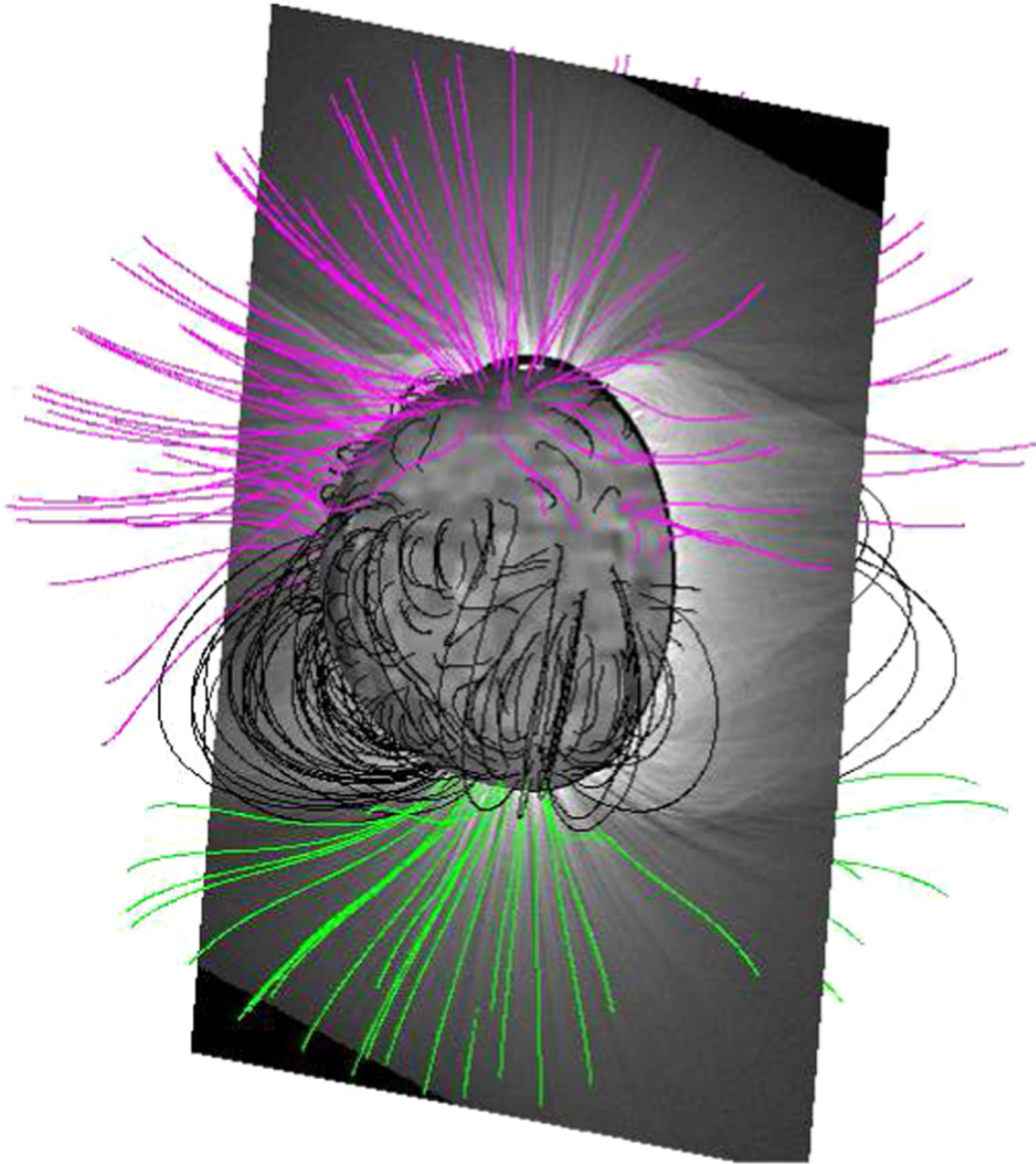
Figure 1. from Image-optimized Coronal Magnetic Field Models null 2017 APJ 844 93 doi:10.3847/1538-4357/aa7b7a https://dx.doi.org/10.3847/1538-4357/aa7b7a © 2017. The American Astronomical Society. All rights reserved.
