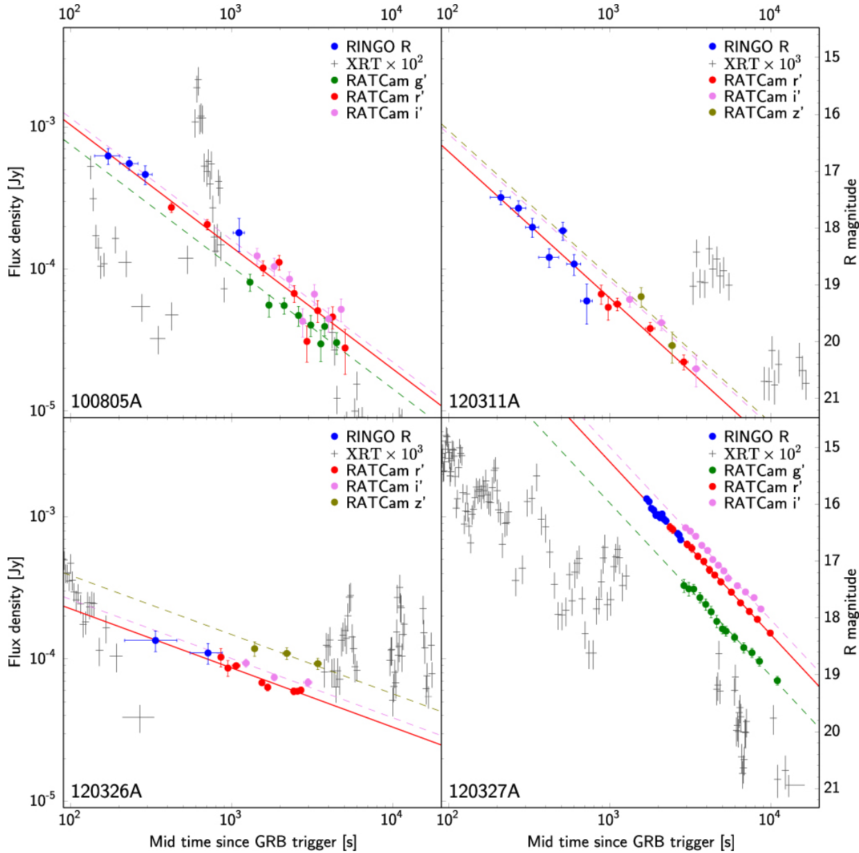
Figure 9. from Polarimetry and Photometry of Gamma-Ray Bursts with RINGO2 null 2017 APJ 843 143 doi:10.3847/1538-4357/aa79a2 https://dx.doi.org/10.3847/1538-4357/aa79a2 © 2017. The American Astronomical Society. All rights reserved.
