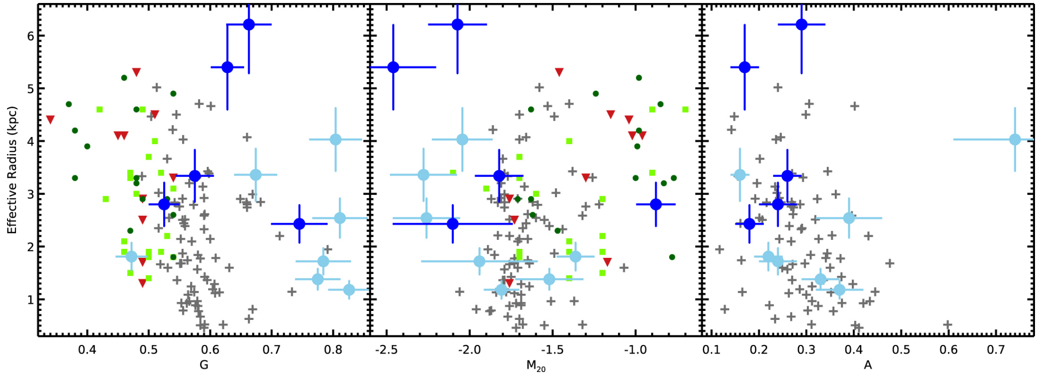
Figure 9. from The Role of the Most Luminous Obscured AGNs in Galaxy Assembly at z \sim 2 null 2017 APJ 844 106 doi:10.3847/1538-4357/aa78f2 https://dx.doi.org/10.3847/1538-4357/aa78f2 © 2017. The American Astronomical Society. All rights reserved.
