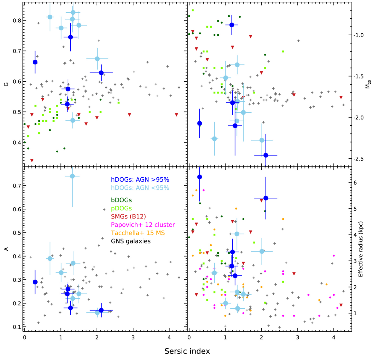
Figure 8. from The Role of the Most Luminous Obscured AGNs in Galaxy Assembly at z \sim 2 null 2017 APJ 844 106 doi:10.3847/1538-4357/aa78f2 https://dx.doi.org/10.3847/1538-4357/aa78f2 © 2017. The American Astronomical Society. All rights reserved.
