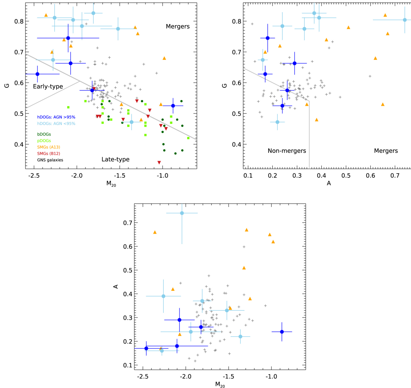
Figure 5. from The Role of the Most Luminous Obscured AGNs in Galaxy Assembly at z \sim 2 null 2017 APJ 844 106 doi:10.3847/1538-4357/aa78f2 https://dx.doi.org/10.3847/1538-4357/aa78f2 © 2017. The American Astronomical Society. All rights reserved.
