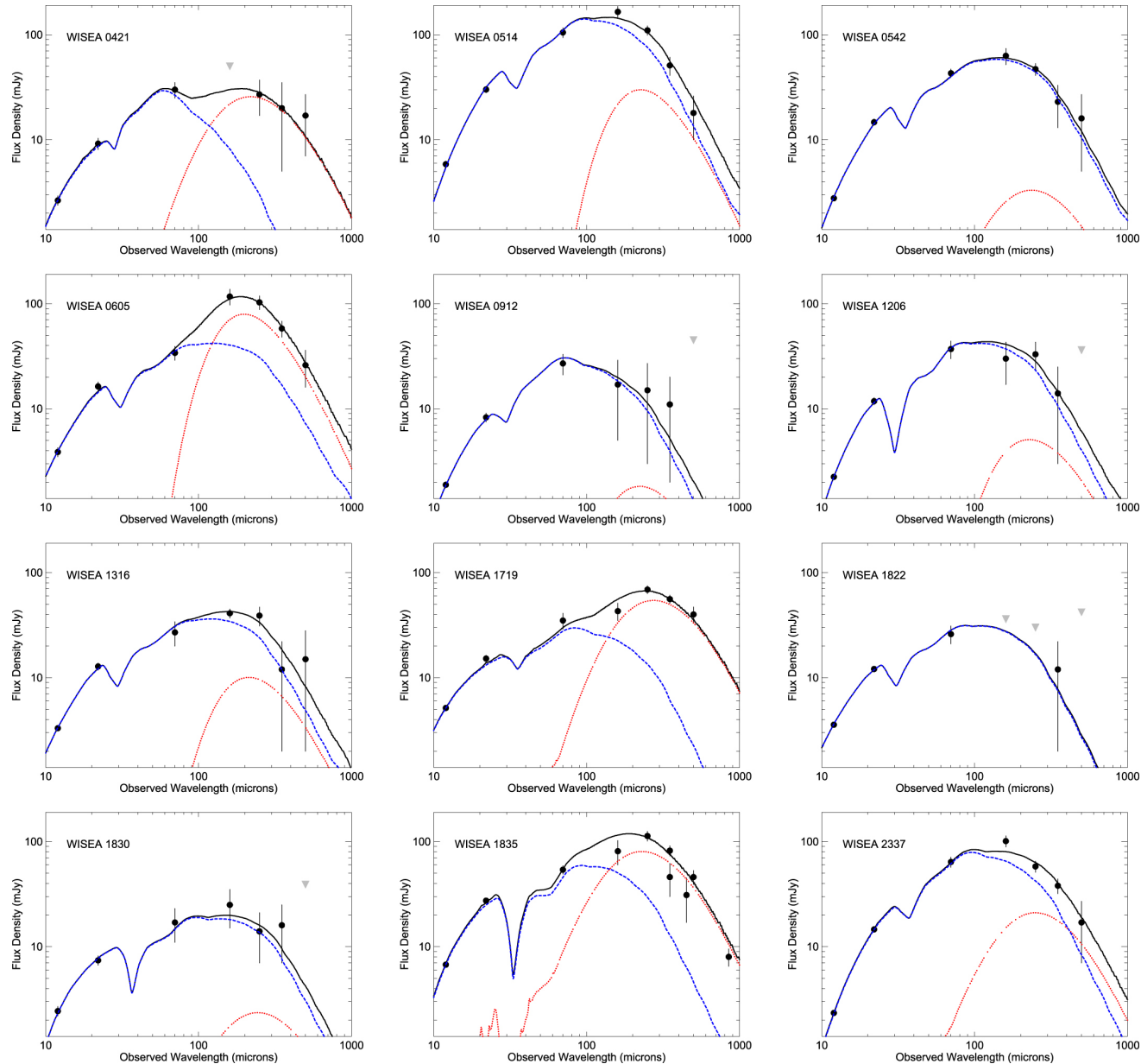
Figure 2. from The Role of the Most Luminous Obscured AGNs in Galaxy Assembly at z \sim 2 null 2017 APJ 844 106 doi:10.3847/1538-4357/aa78f2 https://dx.doi.org/10.3847/1538-4357/aa78f2 © 2017. The American Astronomical Society. All rights reserved.
