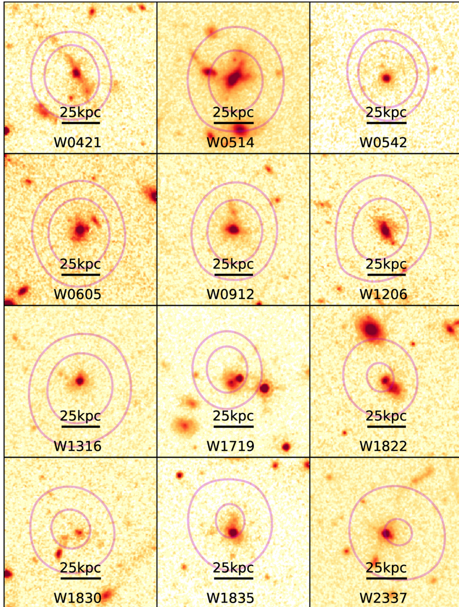
Figure 1. from The Role of the Most Luminous Obscured AGNs in Galaxy Assembly at z \sim 2 null 2017 APJ 844 106 doi:10.3847/1538-4357/aa78f2 https://dx.doi.org/10.3847/1538-4357/aa78f2 © 2017. The American Astronomical Society. All rights reserved.
