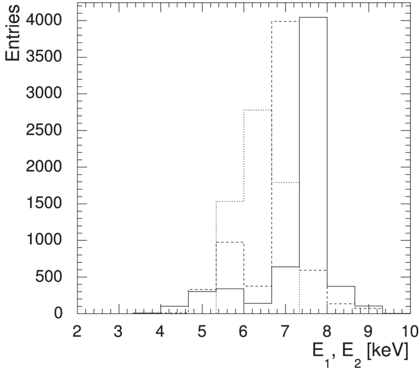
Figure 9. from Simulations of the Fe K Energy Spectra from Gravitationally Microlensed Quasars null 2017 APJ 843 118 doi:10.3847/1538-4357/aa7896 https://dx.doi.org/10.3847/1538-4357/aa7896 © 2017. The American Astronomical Society. All rights reserved.
