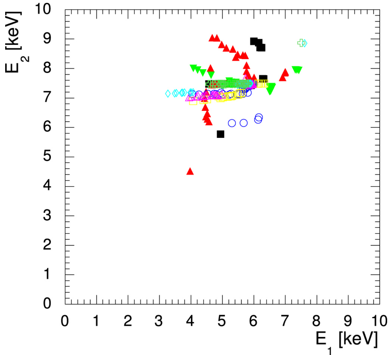
Figure 8. from Simulations of the Fe K Energy Spectra from Gravitationally Microlensed Quasars null 2017 APJ 843 118 doi:10.3847/1538-4357/aa7896 https://dx.doi.org/10.3847/1538-4357/aa7896 © 2017. The American Astronomical Society. All rights reserved.
