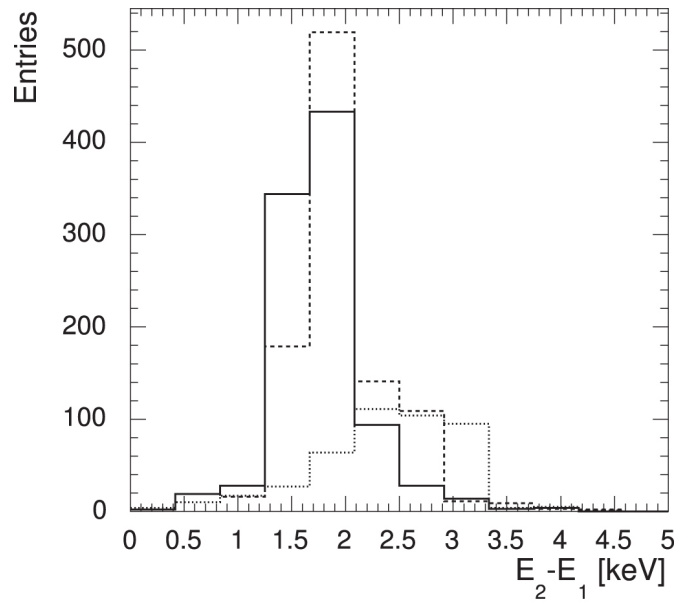
Figure 7. from Simulations of the Fe K Energy Spectra from Gravitationally Microlensed Quasars null 2017 APJ 843 118 doi:10.3847/1538-4357/aa7896 https://dx.doi.org/10.3847/1538-4357/aa7896 © 2017. The American Astronomical Society. All rights reserved.
