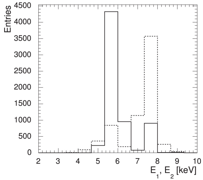
Figure 5. from Simulations of the Fe K Energy Spectra from Gravitationally Microlensed Quasars null 2017 APJ 843 118 doi:10.3847/1538-4357/aa7896 https://dx.doi.org/10.3847/1538-4357/aa7896
