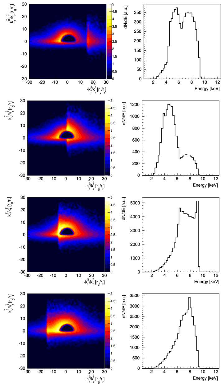
Figure 3. from Simulations of the Fe K Energy Spectra from Gravitationally Microlensed Quasars null 2017 APJ 843 118 doi:10.3847/1538-4357/aa7896 https://dx.doi.org/10.3847/1538-4357/aa7896 © 2017. The American Astronomical Society. All rights reserved.
