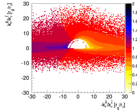
Figure 2. from Simulations of the Fe K Energy Spectra from Gravitationally Microlensed Quasars null 2017 APJ 843 118 doi:10.3847/1538-4357/aa7896 https://dx.doi.org/10.3847/1538-4357/aa7896
