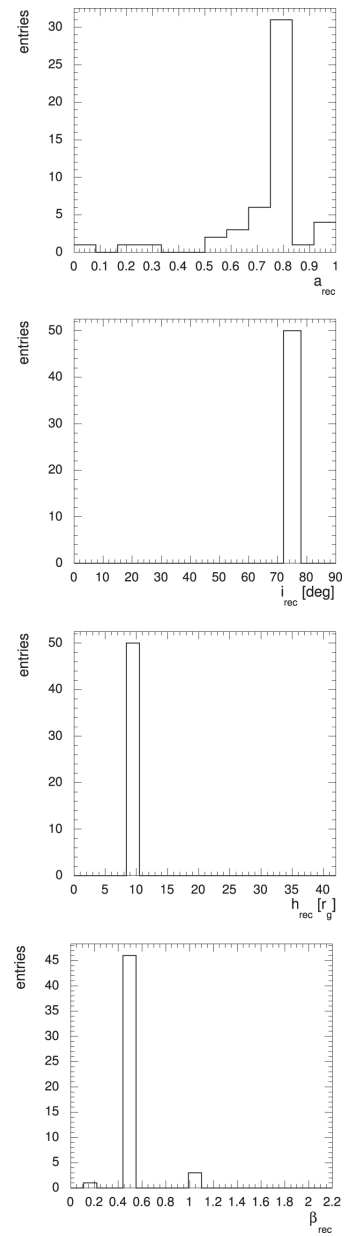
Figure 14. from Simulations of the Fe K Energy Spectra from Gravitationally Microlensed Quasars null 2017 APJ 843 118 doi:10.3847/1538-4357/aa7896 https://dx.doi.org/10.3847/1538-4357/aa7896
