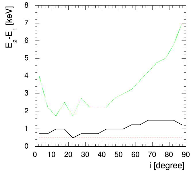
Figure 13. from Simulations of the Fe K Energy Spectra from Gravitationally Microlensed Quasars null 2017 APJ 843 118 doi:10.3847/1538-4357/aa7896 https://dx.doi.org/10.3847/1538-4357/aa7896
