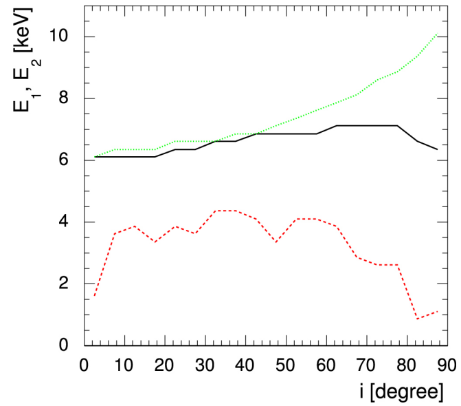
Figure 12. from Simulations of the Fe K Energy Spectra from Gravitationally Microlensed Quasars null 2017 APJ 843 118 doi:10.3847/1538-4357/aa7896 https://dx.doi.org/10.3847/1538-4357/aa7896 © 2017. The American Astronomical Society. All rights reserved.
