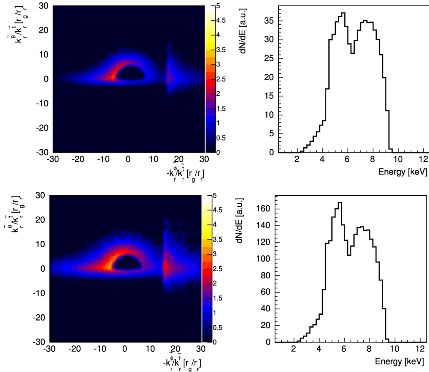
Figure 11. from Simulations of the Fe K Energy Spectra from Gravitationally Microlensed Quasars null 2017 APJ 843 118 doi:10.3847/1538-4357/aa7896 https://dx.doi.org/10.3847/1538-4357/aa7896
