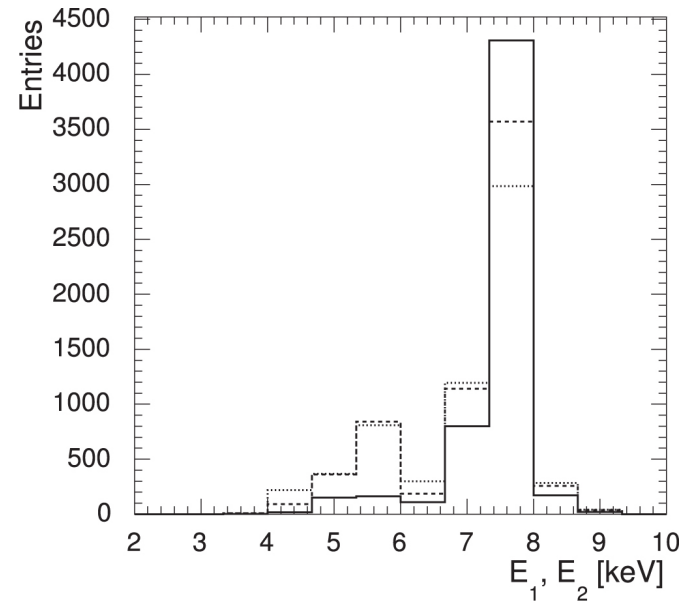
Figure 10. from Simulations of the Fe K Energy Spectra from Gravitationally Microlensed Quasars null 2017 APJ 843 118 doi:10.3847/1538-4357/aa7896 https://dx.doi.org/10.3847/1538-4357/aa7896
