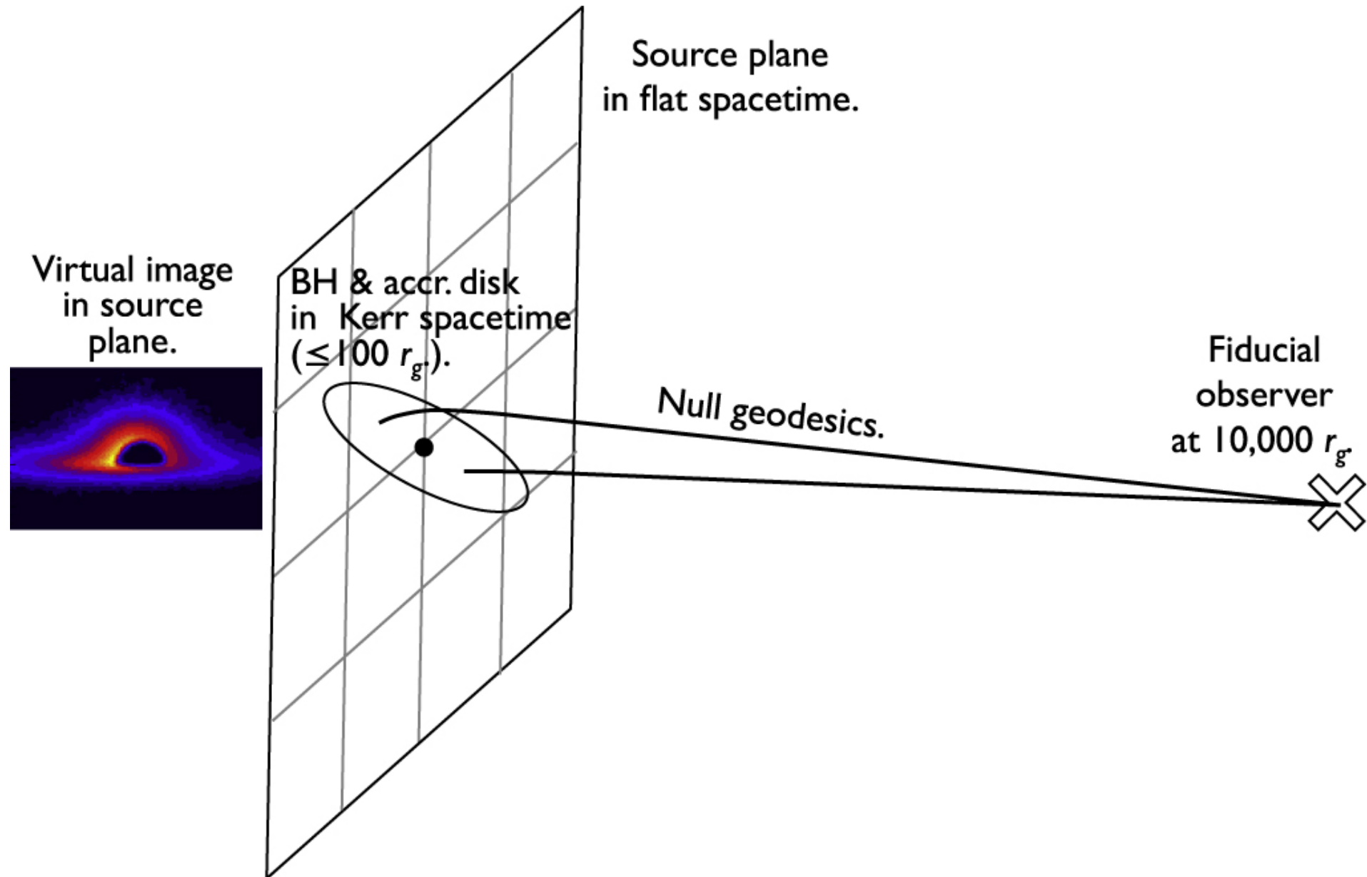
Figure 1. from Simulations of the Fe K Energy Spectra from Gravitationally Microlensed Quasars null 2017 APJ 843 118 doi:10.3847/1538-4357/aa7896 https://dx.doi.org/10.3847/1538-4357/aa7896 © 2017. The American Astronomical Society. All rights reserved.
