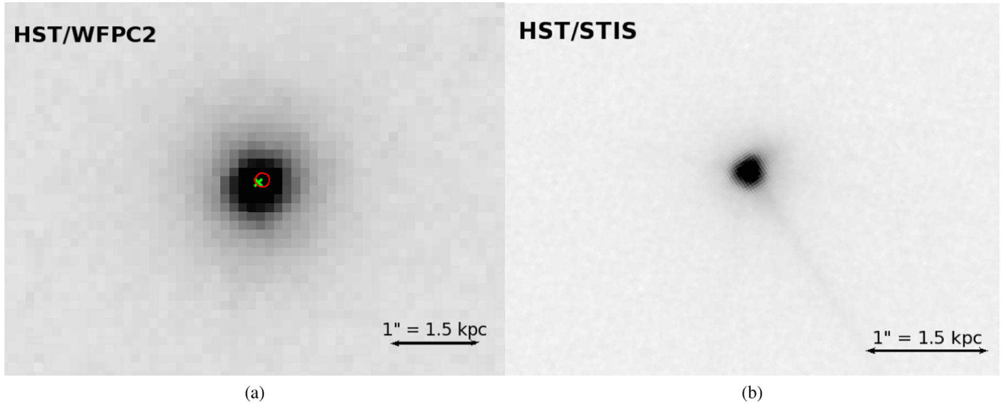
Figure 4. from PS16dtm: A Tidal Disruption Event in a Narrow-line Seyfert 1 Galaxy null 2017 APJ 843 106 doi:10.3847/1538-4357/aa77f7 https://dx.doi.org/10.3847/1538-4357/aa77f7 © 2017. The American Astronomical Society. All rights reserved.
