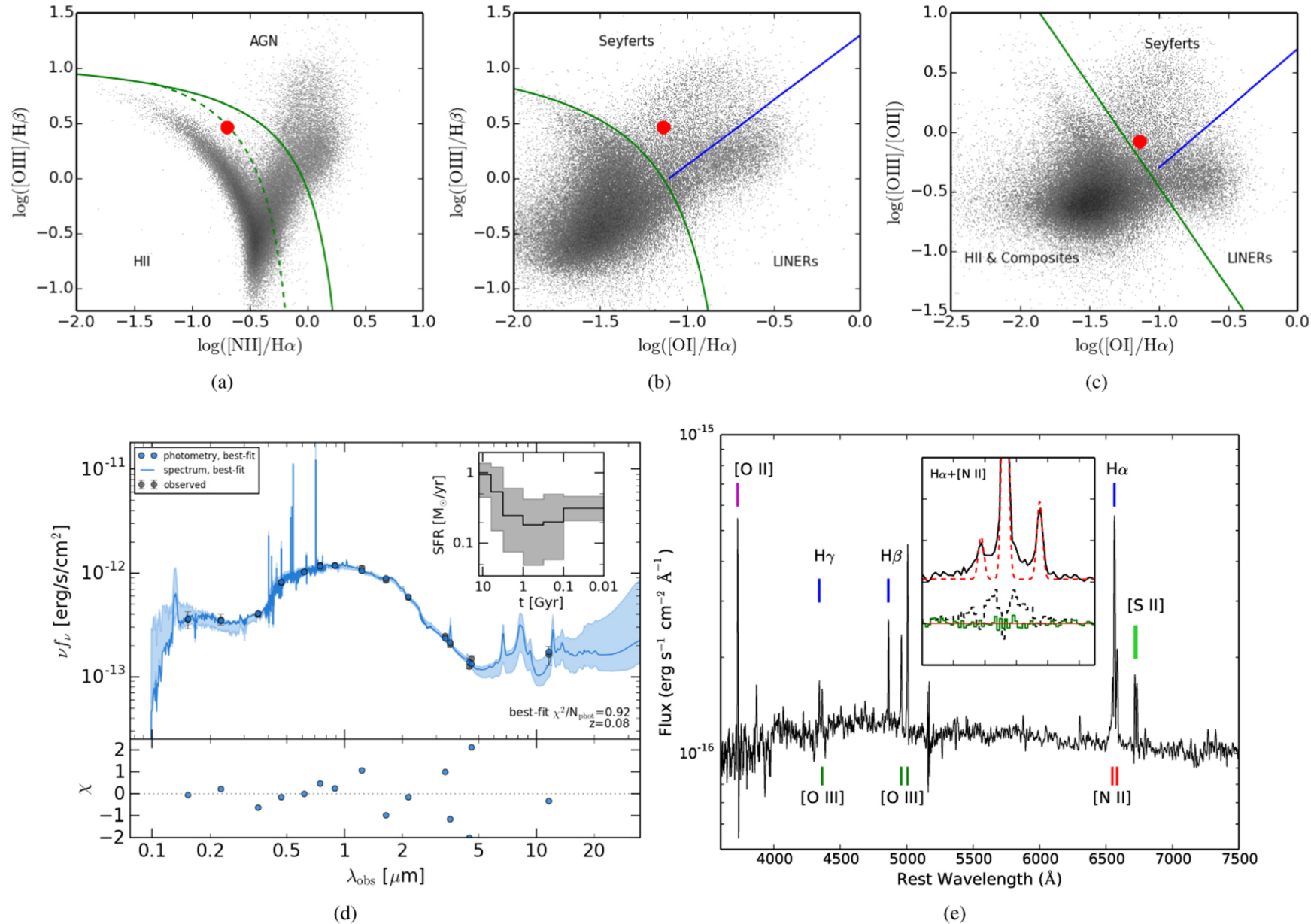
Figure 1. from PS16dtm: A Tidal Disruption Event in a Narrow-line Seyfert 1 Galaxy null 2017 APJ 843 106 doi:10.3847/1538-4357/aa77f7 https://dx.doi.org/10.3847/1538-4357/aa77f7
