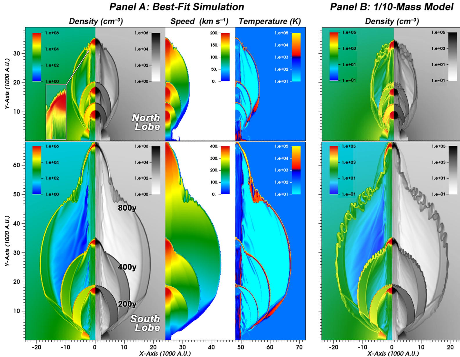
Figure 2. from Models of the Hydrodynamic Histories of Post-AGB Stars. I. Multiflow Shaping of OH 231.8+04.2 null 2017 APJ 843 108 doi:10.3847/1538-4357/aa77f0 https://dx.doi.org/10.3847/1538-4357/aa77f0
