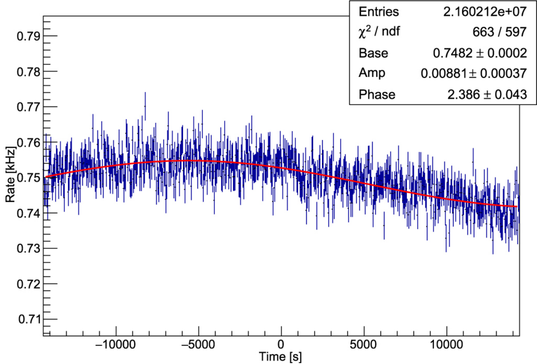
Figure 1. from Search for Very-high-energy Emission from Gamma-Ray Bursts Using the First 18 Months of Data from the HAWC Gamma-Ray Observatory null 2017 APJ 843 88 doi:10.3847/1538-4357/aa756f https://dx.doi.org/10.3847/1538-4357/aa756f © 2017. The American Astronomical Society. All rights reserved.
