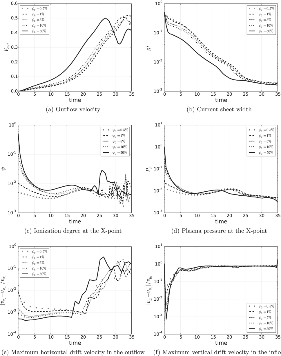
Figure 9. from Effect of Radiation on Chromospheric Magnetic Reconnection: Reactive and Collisional Multi-fluid Simulations null 2017 APJ 842 117 doi:10.3847/1538-4357/aa7554 https://dx.doi.org/10.3847/1538-4357/aa7554
