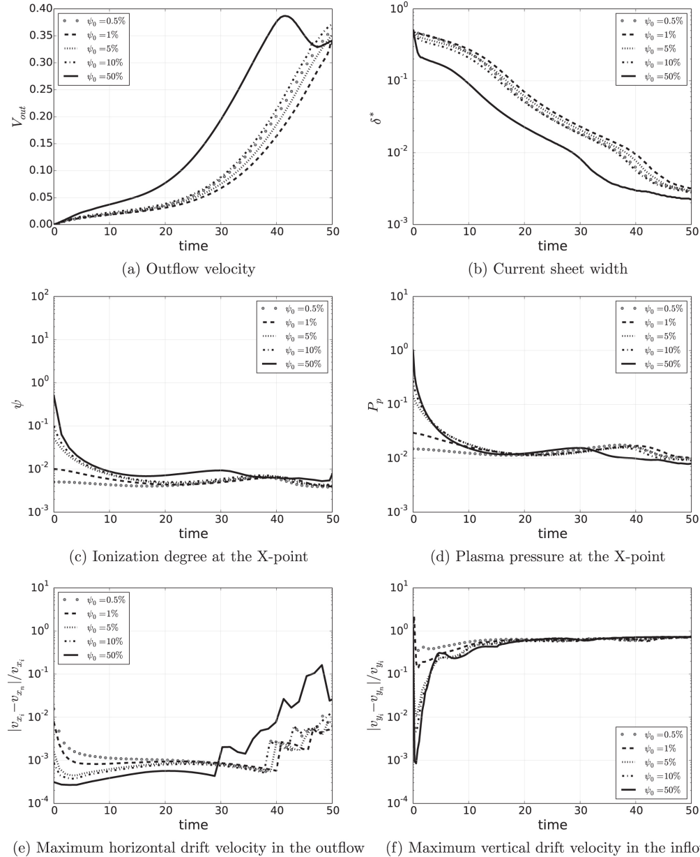
Figure 6. from Effect of Radiation on Chromospheric Magnetic Reconnection: Reactive and Collisional Multi-fluid Simulations null 2017 APJ 842 117 doi:10.3847/1538-4357/aa7554 https://dx.doi.org/10.3847/1538-4357/aa7554
