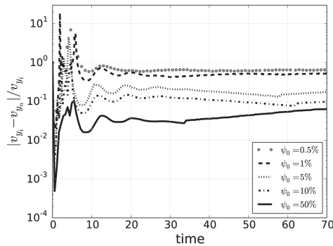
(f) Maximum vertical drift velocity in the inflow
