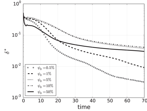
(b) Current sheet width
