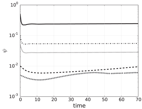
(c) Ionization degree at the X-point
