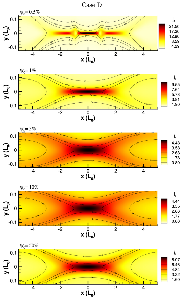
Figure 10. from Effect of Radiation on Chromospheric Magnetic Reconnection: Reactive and Collisional Multi-fluid Simulations null 2017 APJ 842 117 doi:10.3847/1538-4357/aa7554 https://dx.doi.org/10.3847/1538-4357/aa7554 © 2017. The American Astronomical Society. All rights reserved.
