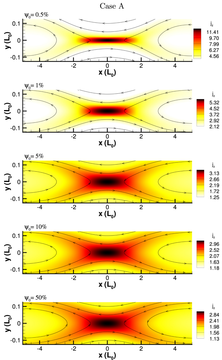
Figure 1. from Effect of Radiation on Chromospheric Magnetic Reconnection: Reactive and Collisional Multi-fluid Simulations null 2017 APJ 842 117 doi:10.3847/1538-4357/aa7554 https://dx.doi.org/10.3847/1538-4357/aa7554 © 2017. The American Astronomical Society. All rights reserved.
