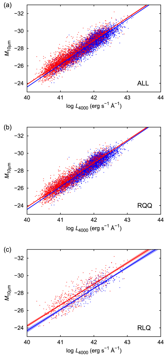
Figure 8. from Properties of Spectrally Defined Red QSOs at z = 0.3\text{--}1.2 null 2017 APJ 842 57 doi:10.3847/1538-4357/aa745b https://dx.doi.org/10.3847/1538-4357/aa745b © 2017. The American Astronomical Society. All rights reserved.
