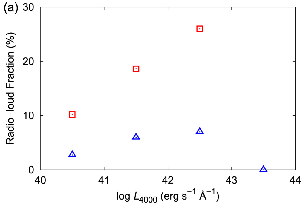
Figure 6. from Properties of Spectrally Defined Red QSOs at z = 0.3\text{--}1.2 null 2017 APJ 842 57 doi:10.3847/1538-4357/aa745b https://dx.doi.org/10.3847/1538-4357/aa745b © 2017. The American Astronomical Society. All rights reserved.
