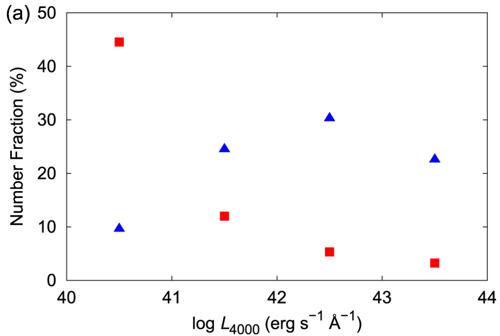
Figure 5. from Properties of Spectrally Defined Red QSOs at z = 0.3\text{--}1.2 null 2017 APJ 842 57 doi:10.3847/1538-4357/aa745b https://dx.doi.org/10.3847/1538-4357/aa745b © 2017. The American Astronomical Society. All rights reserved.
