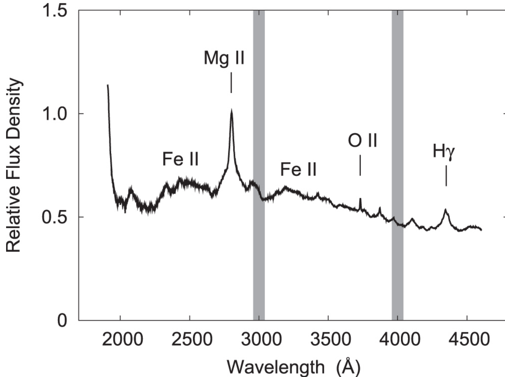
Figure 1. from Properties of Spectrally Defined Red QSOs at z = 0.3\text{--}1.2 null 2017 APJ 842 57 doi:10.3847/1538-4357/aa745b https://dx.doi.org/10.3847/1538-4357/aa745b © 2017. The American Astronomical Society. All rights reserved.
