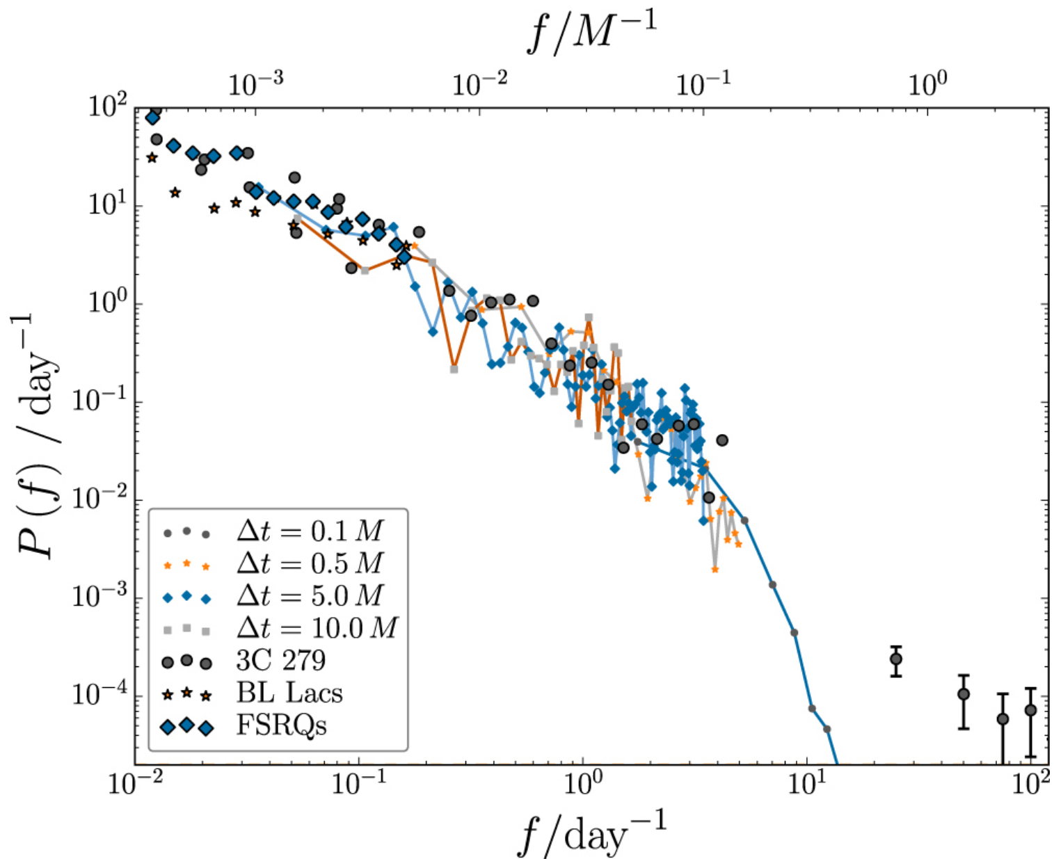
Figure 5. from Blazar Variability from Turbulence in Jets Launched by Magnetically Arrested Accretion Flows null 2017 APJ 843 81 doi:10.3847/1538-4357/aa7339 https://dx.doi.org/10.3847/1538-4357/aa7339 © 2017. The American Astronomical Society. All rights reserved.
