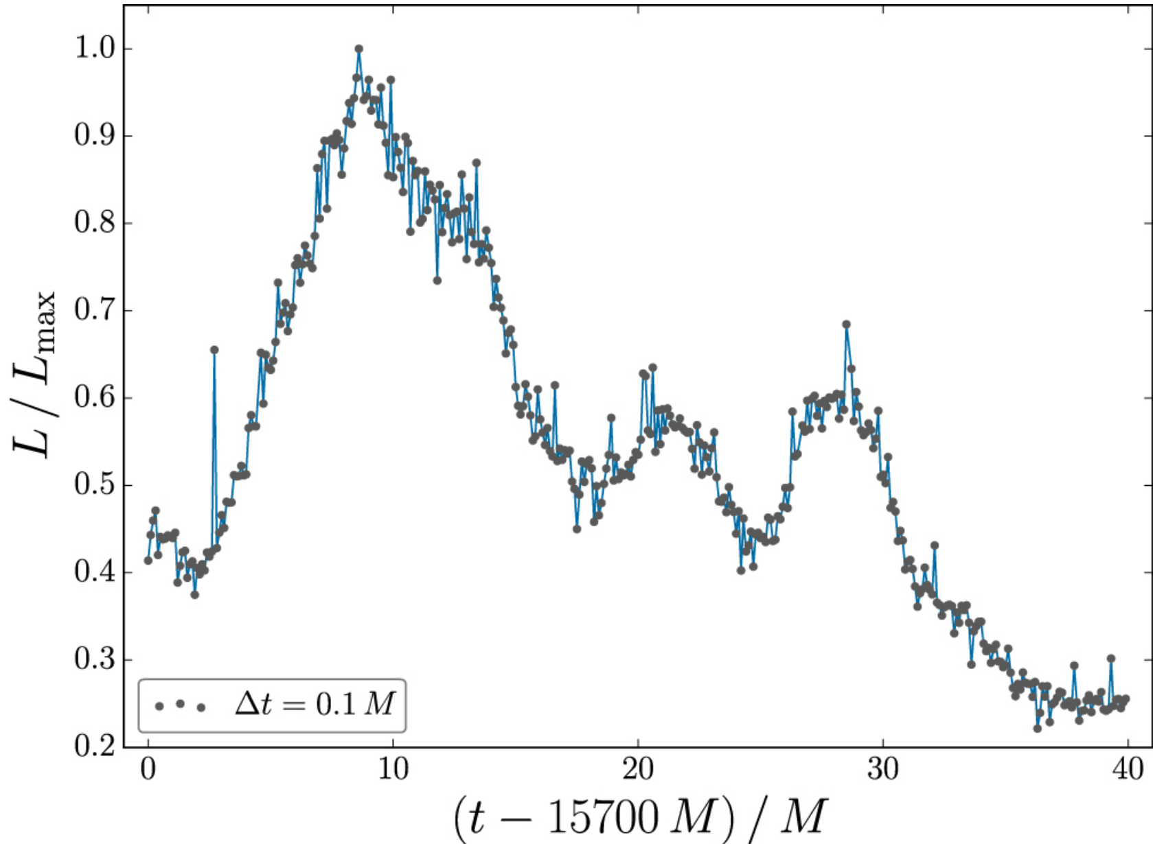
Figure 4. from Blazar Variability from Turbulence in Jets Launched by Magnetically Arrested Accretion Flows null 2017 APJ 843 81 doi:10.3847/1538-4357/aa7339 https://dx.doi.org/10.3847/1538-4357/aa7339 © 2017. The American Astronomical Society. All rights reserved.
