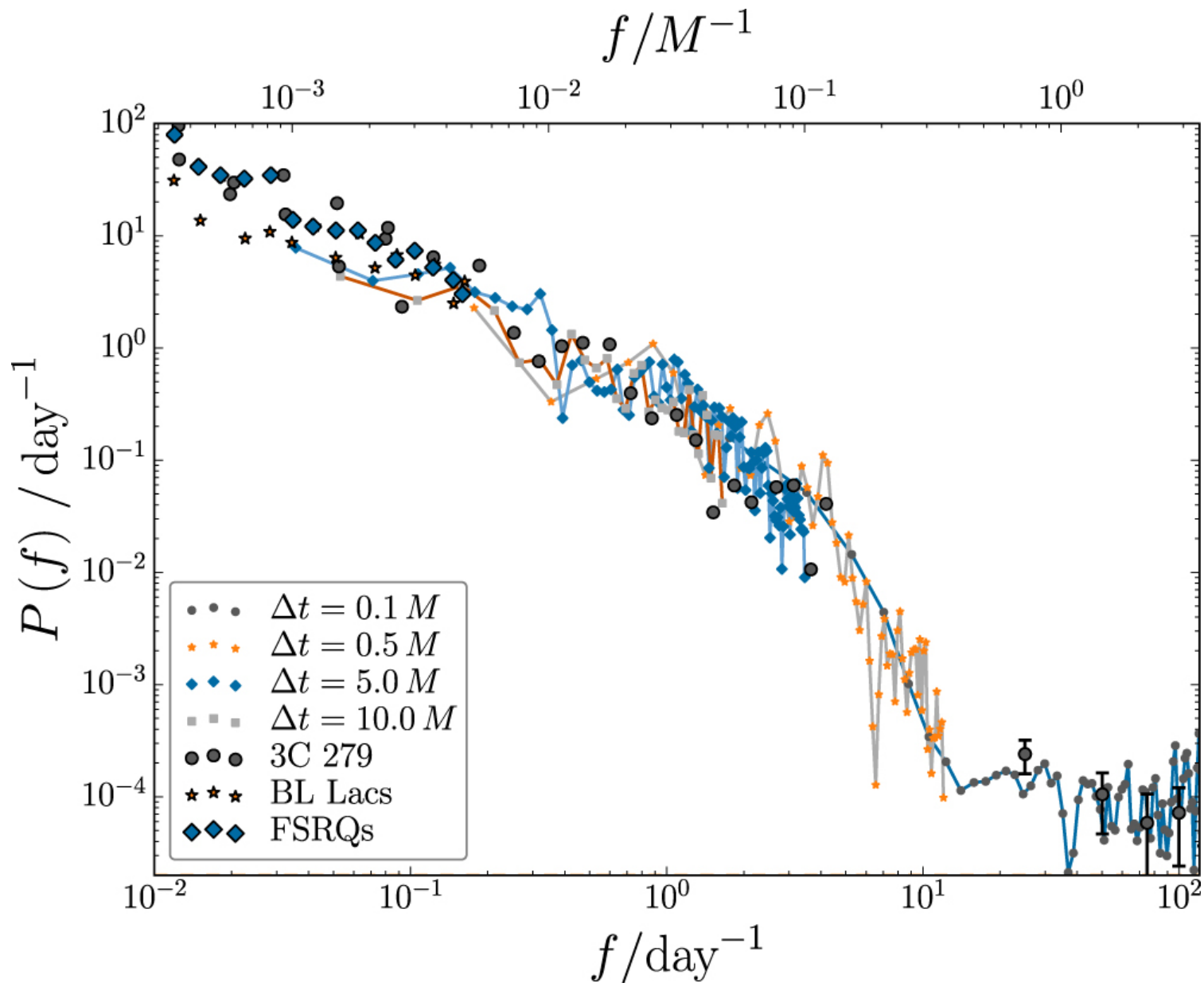
Figure 3. from Blazar Variability from Turbulence in Jets Launched by Magnetically Arrested Accretion Flows null 2017 APJ 843 81 doi:10.3847/1538-4357/aa7339 https://dx.doi.org/10.3847/1538-4357/aa7339 © 2017. The American Astronomical Society. All rights reserved.
