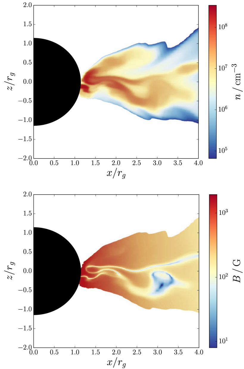
Figure 2. from Blazar Variability from Turbulence in Jets Launched by Magnetically Arrested Accretion Flows null 2017 APJ 843 81 doi:10.3847/1538-4357/aa7339 https://dx.doi.org/10.3847/1538-4357/aa7339 © 2017. The American Astronomical Society. All rights reserved.
