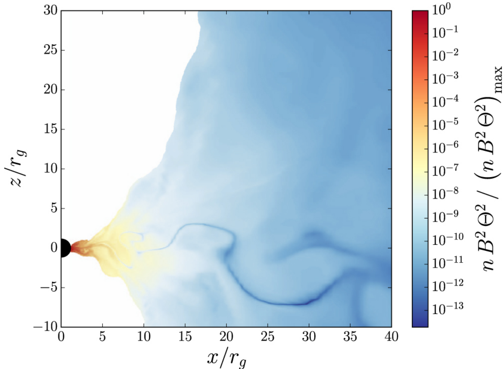
Figure 1. from Blazar Variability from Turbulence in Jets Launched by Magnetically Arrested Accretion Flows null 2017 APJ 843 81 doi:10.3847/1538-4357/aa7339 https://dx.doi.org/10.3847/1538-4357/aa7339 © 2017. The American Astronomical Society. All rights reserved.
