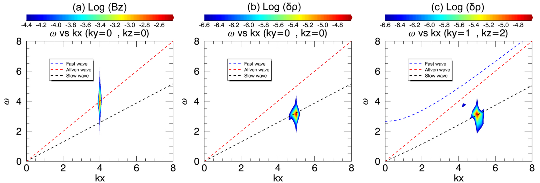
Figure 8. from The Parametric Decay Instability of Alfvén Waves in Turbulent Plasmas and the Applications in the Solar Wind null 2017 APJ 842 63 doi:10.3847/1538-4357/aa71b6 https://dx.doi.org/10.3847/1538-4357/aa71b6 © 2017. The American Astronomical Society. All rights reserved.
